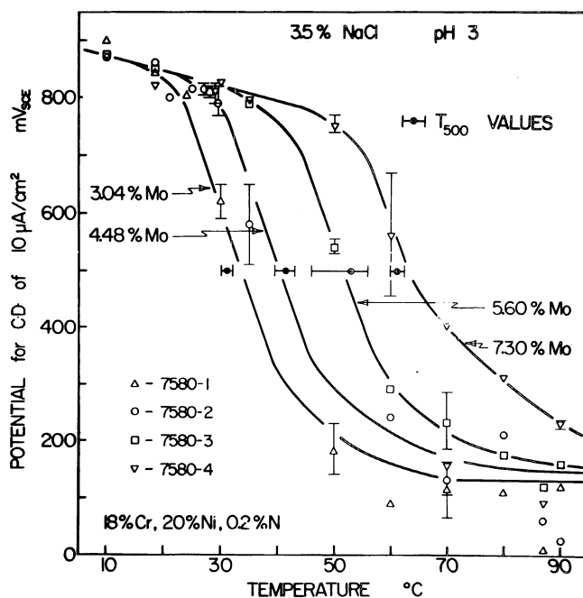
FIGURE 2 – Comparison of increasing potential runs (open symbols) and increasing temperature ( T_{500} ) values for a series of 18% Cr, 20% Ni, 0.2% N stainless steels.
